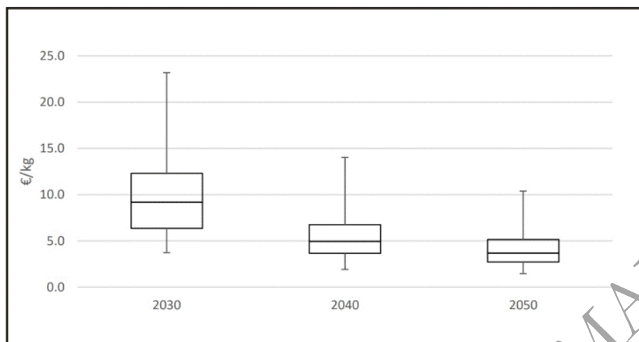
Figure 4 Range of hydrogen production costs due to parameter variation 3 . (Source: Energieinstitut an der JKU Linz)
