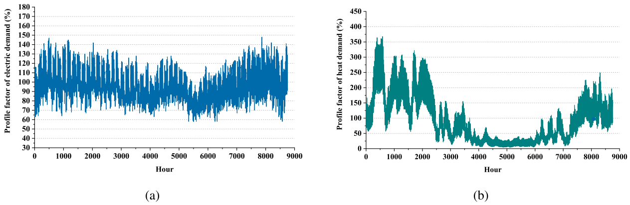
Fig. 4. Profile factors of electricity and heat consumption in the Netherlands.
